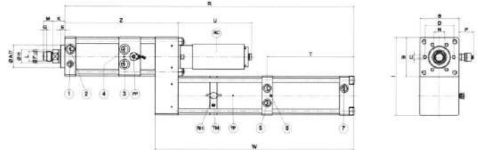
Picture 1 _Unit view, attention to keep air at the hole n. 5 Version “E”
