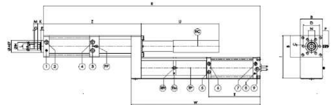
Picture 1.1 unit view, attention to keep air at the hole n. 5 version “NG”
