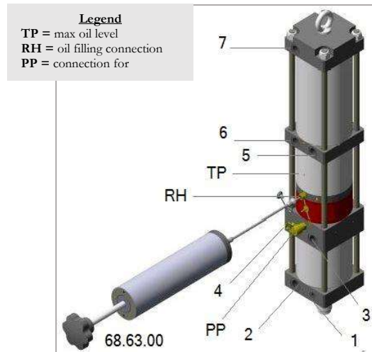
Picture 6 _ Connection of oil filling pump
